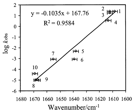
FIGURE 6: Plot of \nu_{\text{C=O}} frequencies vs the single-turnover rate ( \log k_{\text{obs}} ) for the 4-CBA-CoA dehalogenase series. (1) 4-CBA-CoA-D145A: 1608 \text{cm}^{-1} , k_{\text{obs}}(\text{WT}) = 24 \text{ s}^{-1} . (2) 4-MBA-CoA-WT: 1612 \text{cm}^{-1} , k_{\text{obs}} = 24 \text{ s}^{-1} . (3) 4-MBA-CoA-A112V: 1612 \text{cm}^{-1} , k_{\text{obs}} = 17 \text{ s}^{-1} . (4) 4-MBA-CoA-Y65D: 1613 \text{cm}^{-1} , k_{\text{obs}} = 3.4 \text{ s}^{-1} . (5) 4-MBA-CoA-G113A: 1638 \text{cm}^{-1} , k_{\text{obs}} = 4.5 \times 10^{-3} \text{ s}^{-1} . (6) 4-CBA-CoA-G113S: 1639 \text{cm}^{-1} , k_{\text{obs}} = 8.5 \times 10^{-4} \text{ s}^{-1} . (7) 4-MBA-CoA-G113S: 1655 \text{cm}^{-1} , k_{\text{obs}} = 8.5 \times 10^{-4} \text{ s}^{-1} . (8) 4-MBA-CoA-F64P: 1668 \text{cm}^{-1} , k_{\text{obs}} = 1 \times 10^{-5} \text{ s}^{-1} . (9) 4-CBA-CoA-F64P: 1667 \text{cm}^{-1} , k_{\text{obs}} = 1 \times 10^{-5} \text{ s}^{-1} . (10) 4-CBA-CoA-G113N: 1669 \text{cm}^{-1} , k_{\text{obs}} = 3.9 \times 10^{-5} \text{ s}^{-1} . The solid line represents a linear regression fit to the data with a correlation coefficient R^2 of 0.9584. The error bars denote the accuracy of \text{C=O} frequency positions ( 2 \text{ cm}^{-1} ).
